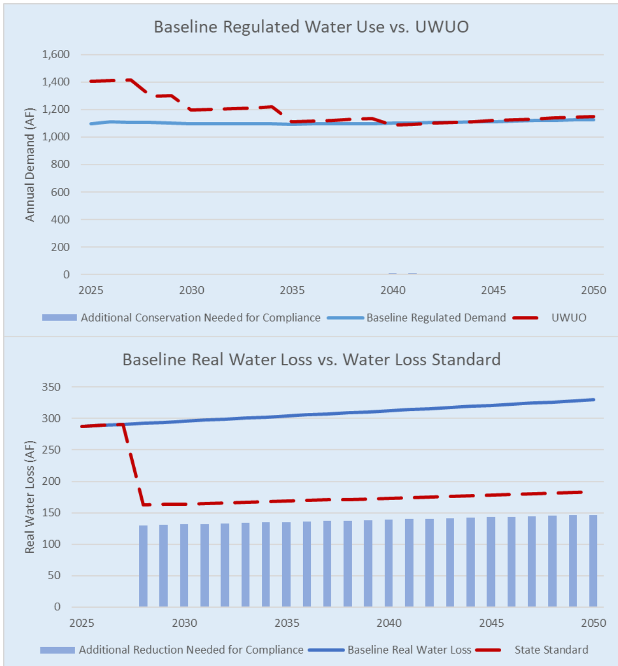
Figure 11. Dixon District Projected Regulated Demands & Real Water Loss
