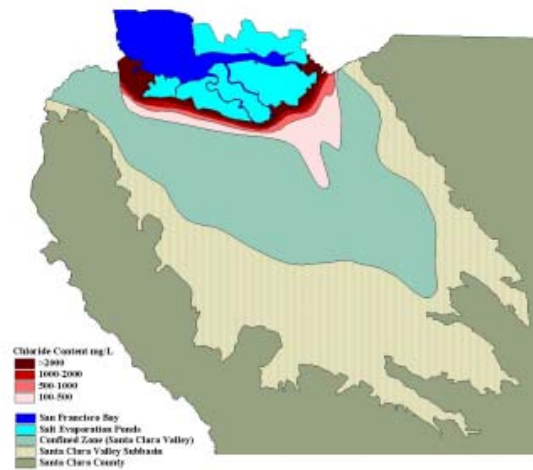
Figure 5-3 Upper Zone Saltwater Intrusion
