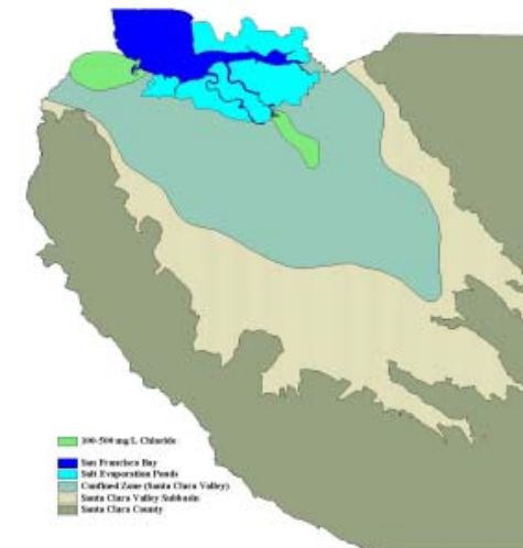
Figure 5-4 Lower Zone Saltwater Intrusion
