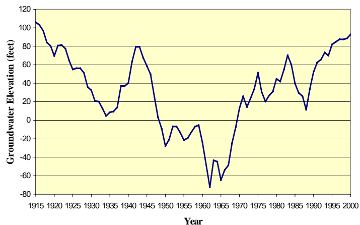
Figure 2-4 Groundwater Elevations in San Jose Index Well
