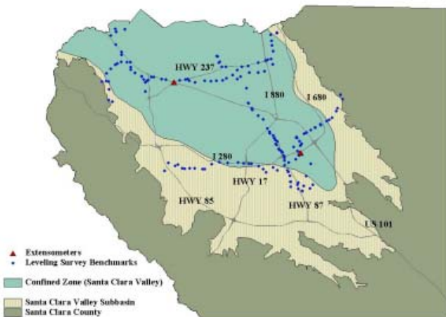
Figure 4-3 Location of Extensometers and Leveling Survey Benchmarks
